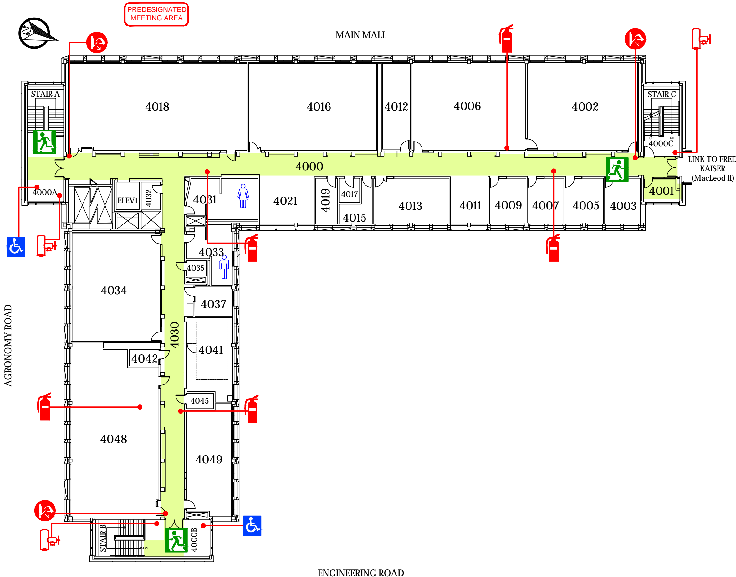
FOURTH FLOOR PLAN N.T.S.
